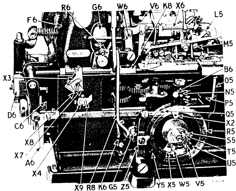
Fig. 9. "X-Ray" View of Pattern Wheel Showing Tripping Points
