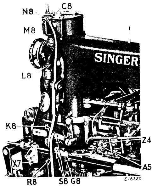
Fig. 34. Adjustment of Automatic Needle Thread Tension Releaser
