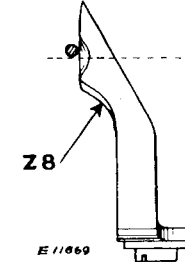
Fig. 17. Showing Correct Relative Positions of Right Hand Loop Retainer and Needle
