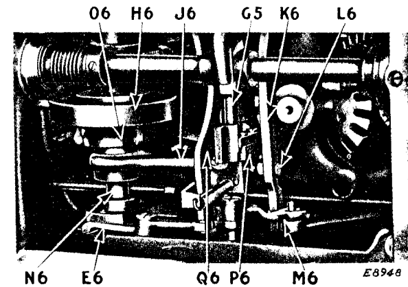
Fig. 19. Rapid Feed Suspended
