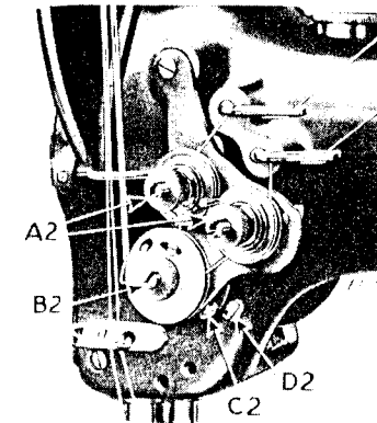
Fig. 15. Adjustment of Thread Controller
