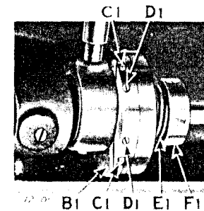
Fig. 19. The Feed Eccentric
