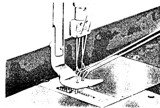
Fig. 11. Drawing Up the Bobbin Threads
