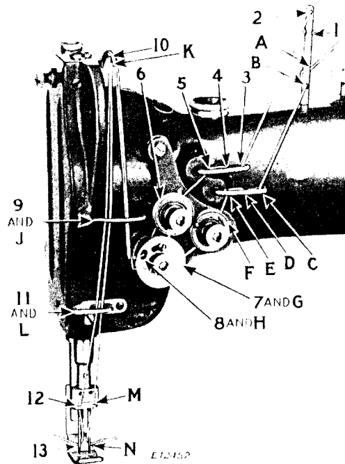
Fig. 10. Upper Threading
