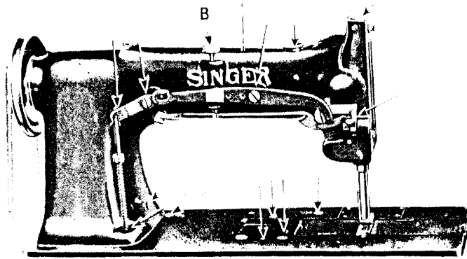
Fig. 3. Oiling Points at the Back of the Machine
