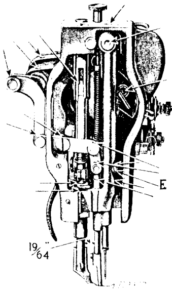
Fig. 13 End View of Machine 111w104 Showing Oiling Points
