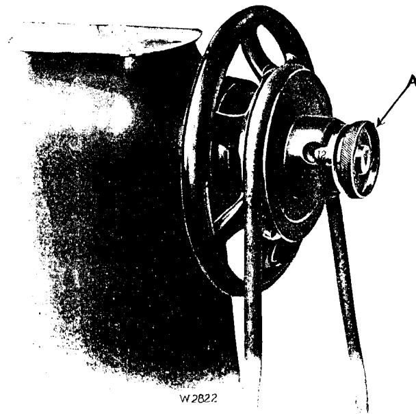
Fig. 11. Stitch Regulator
