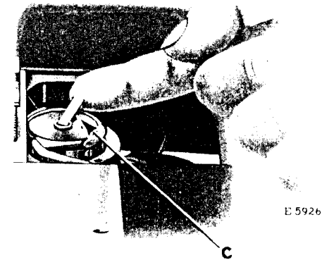
Fig. 3. Removing the Bobbin
