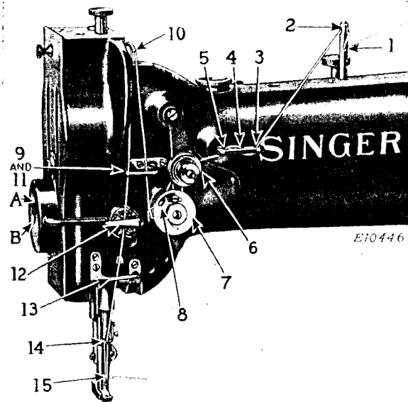
Fig. 7. Upper Threading
