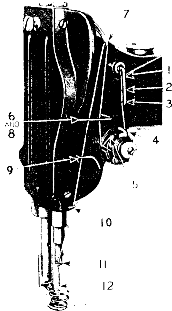
Fig. 7. Upper Threading
